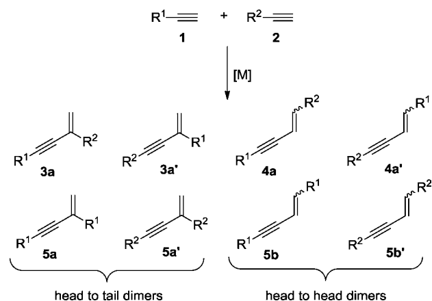
Scheme 1. Possible Products from Dimerization of Two Terminal Alkynes
