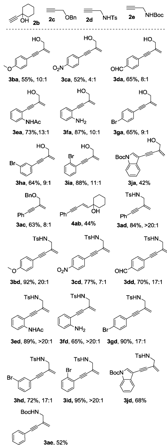
Figure 1. Rhodium-catalyzed cross-dimerization of arylacetylenes and propargylic alcohols, ethers, or amides. Reaction conditions: arylacetylene 1 (0.5 mmol), propargylic alcohol/ether/amide 2 (0.75 mmol), [\text{Rh}(\text{COD})\text{Cl}]_2 (5 mol %), \text{Ph}_3\text{P} (20 mol %), DCM (1 mL), 40 °C, overnight. The ratio of two heterodimers was determined by ^1\text{H} NMR of the purified mixtures of isomers after column chromatography, and the yields were the isolated yield of two isomers.
